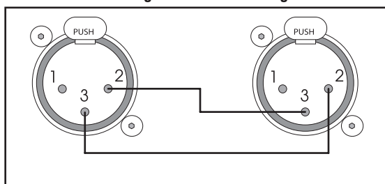
Bridged Mode XLR Wiring
